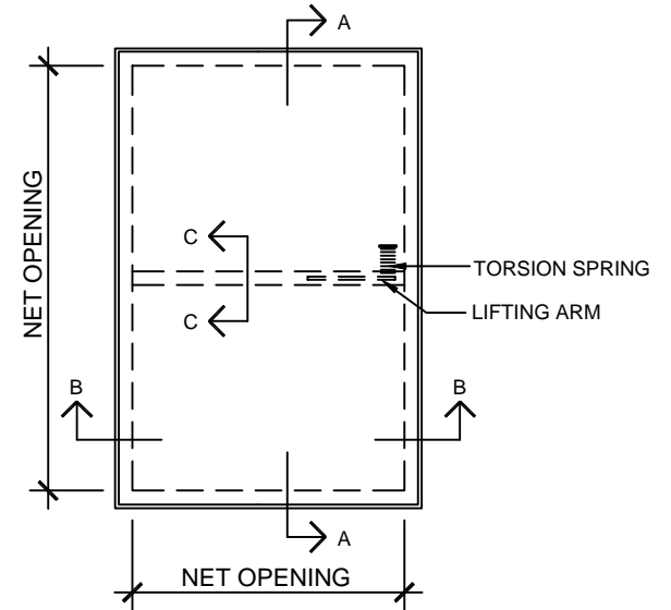
PLAN VIEW- SV NOT TO SCALE
